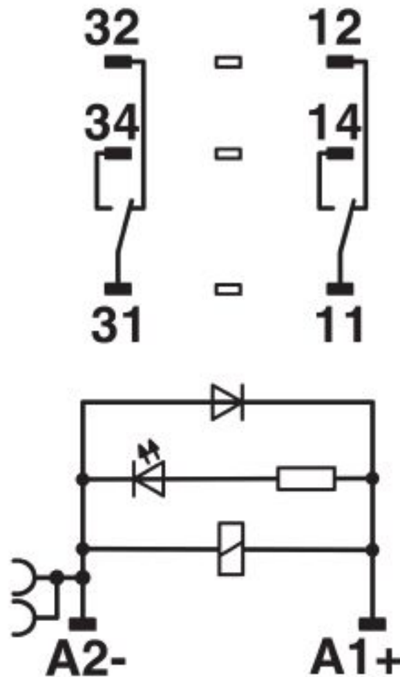
Circuit diagram
