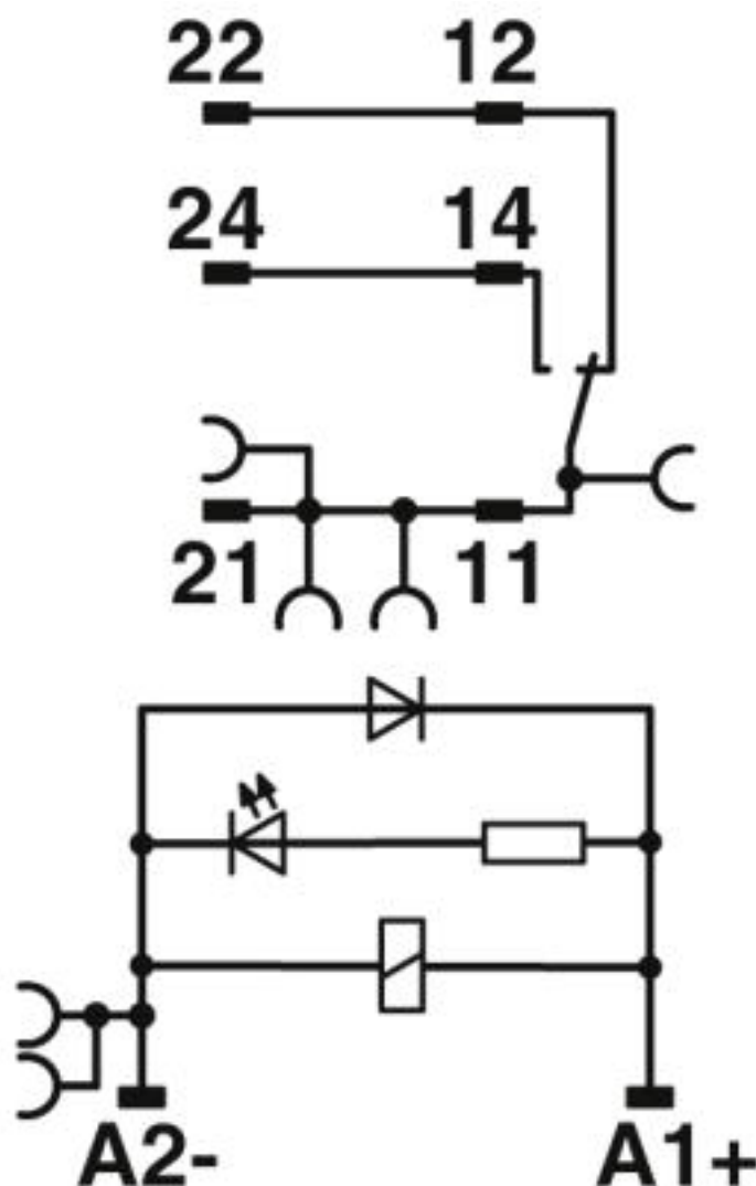
Circuit diagram
