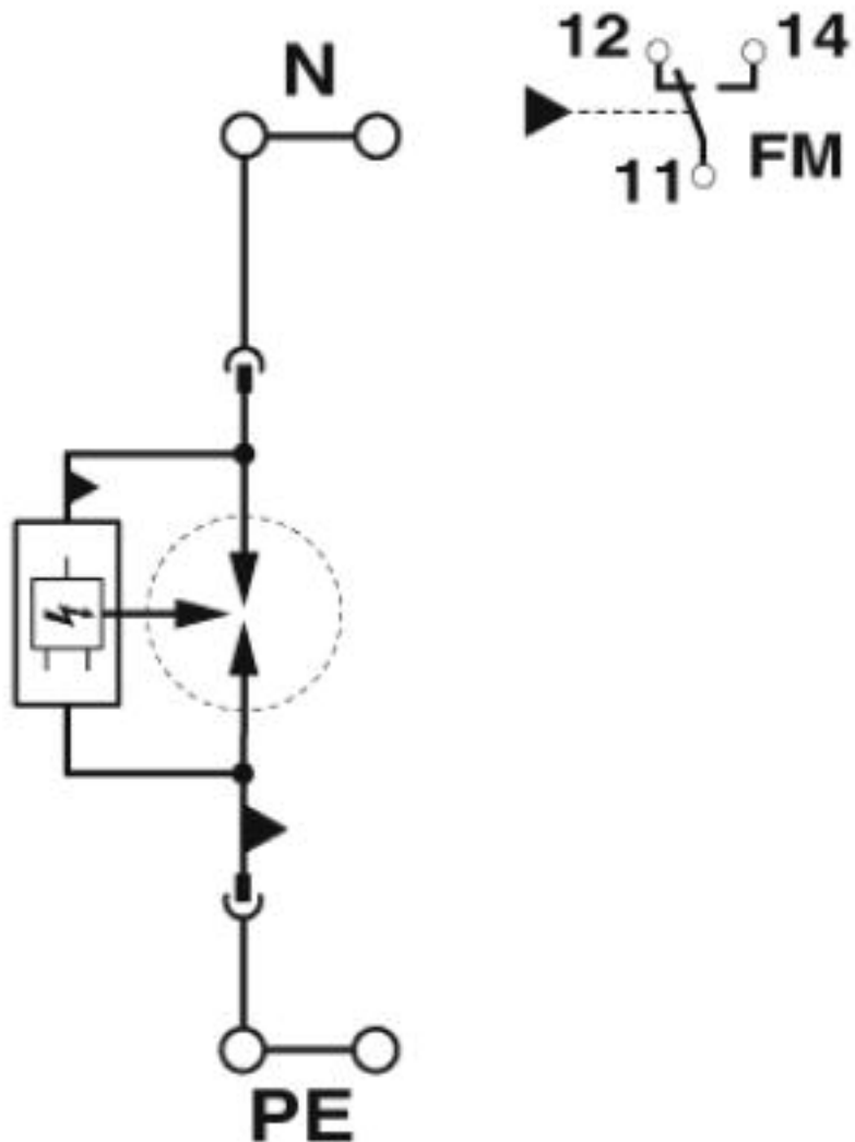
Circuit diagram
