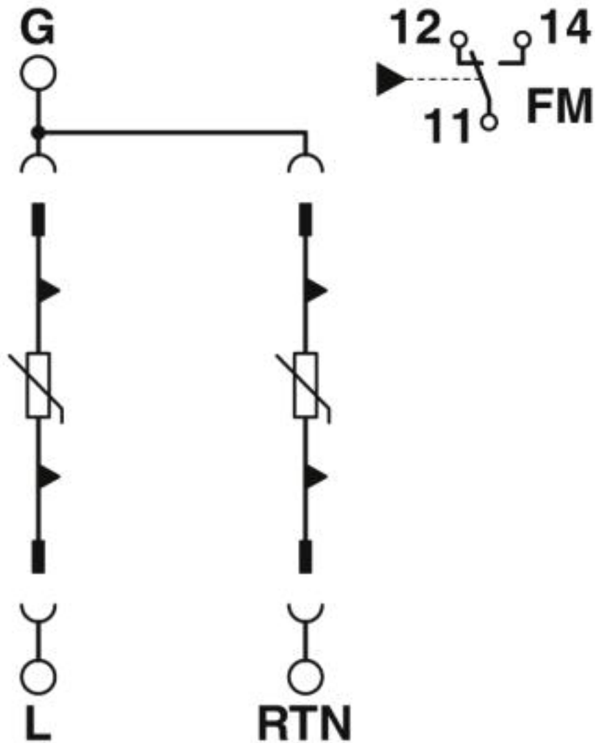
Circuit diagram
