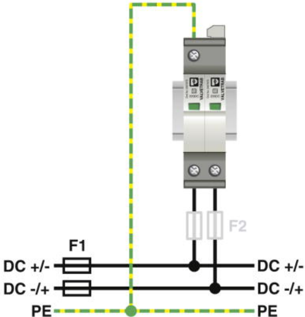
Application drawing
