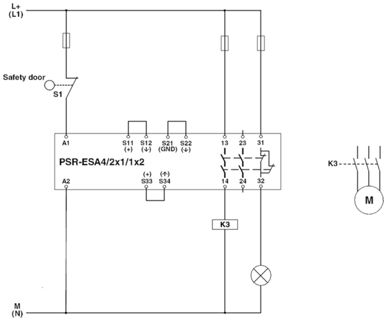
Circuit diagram
