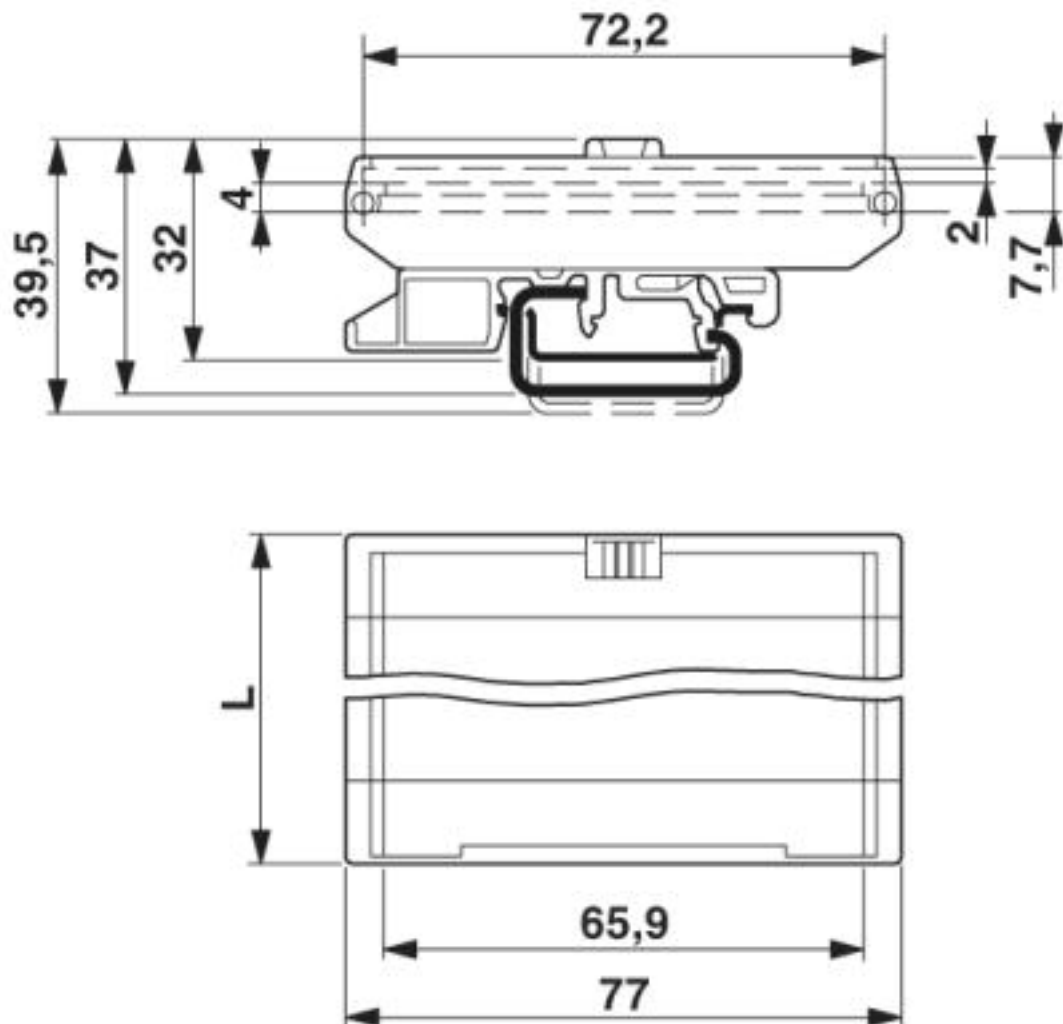
Dimensional drawing
