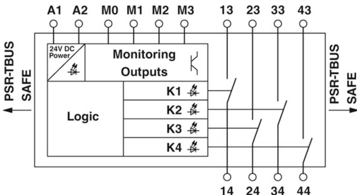
Circuit diagram
