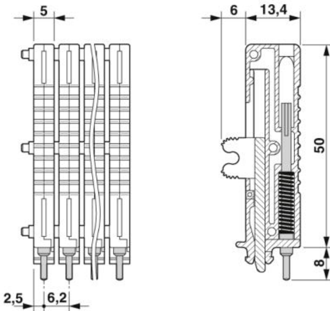
Dimensional drawing
