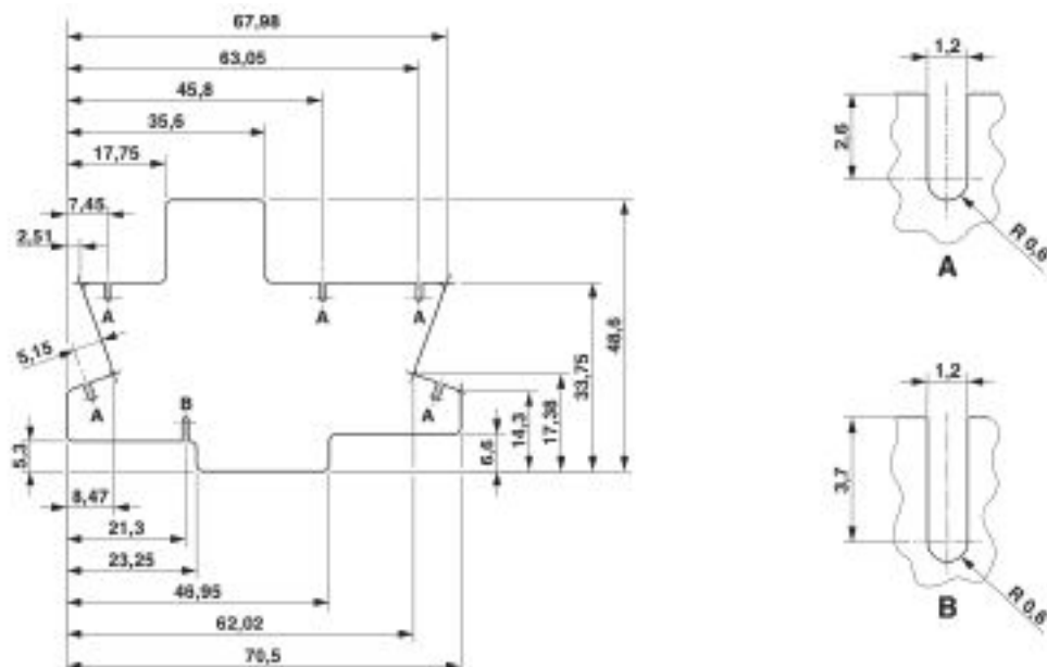
Dimensional drawing
