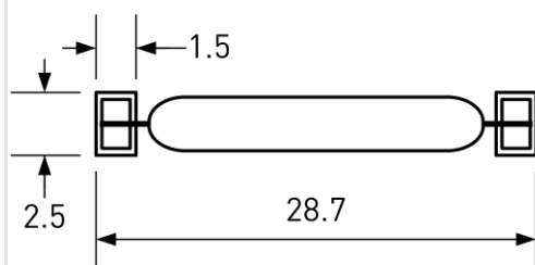
Pad sizes
