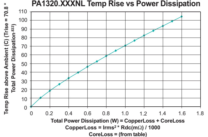
PA1320.XXXNL Temp Rise vs Power Dissipation
