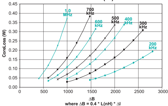
CoreLoss (W)
