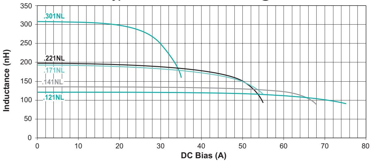
Typical Inducance vs DC Bias @ 25°C
