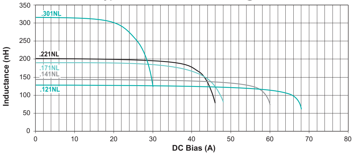
Typical Inducance vs DC Bias @ 100°C
