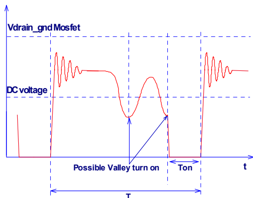
Valley Switching at heavy load
