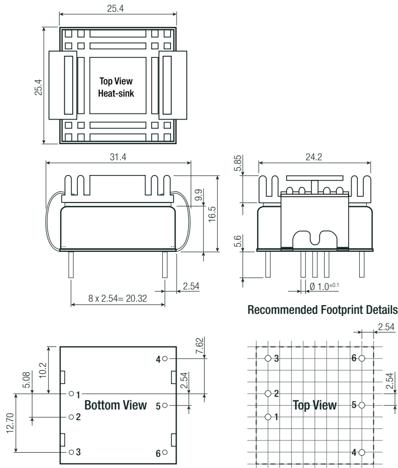
Dimension Drawing with Heat-sink (mm)
