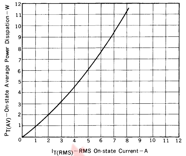
Fig. 10 P_{T(AV)} - I_T(\text{RMS}) CHARACTERISTIC
