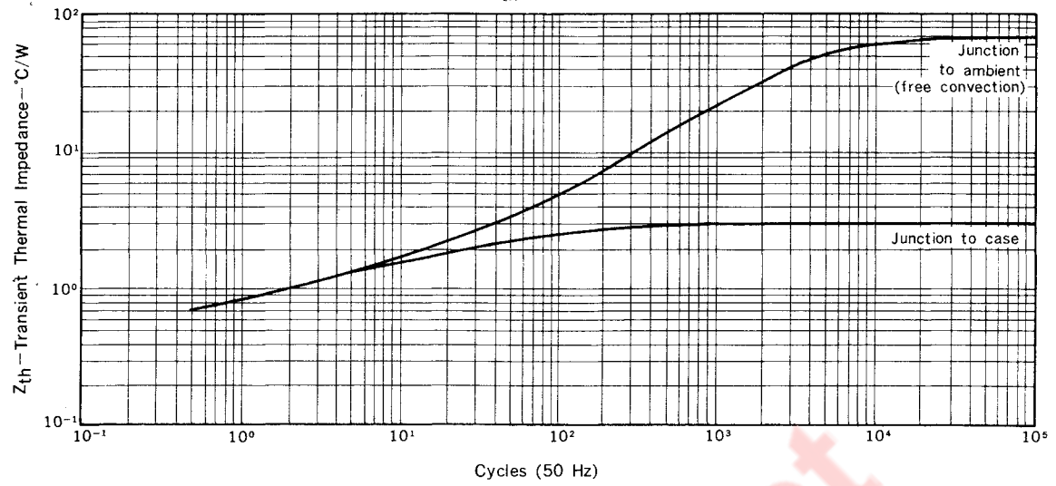
Fig. 13 Z_{th} CHARACTERISTIC
