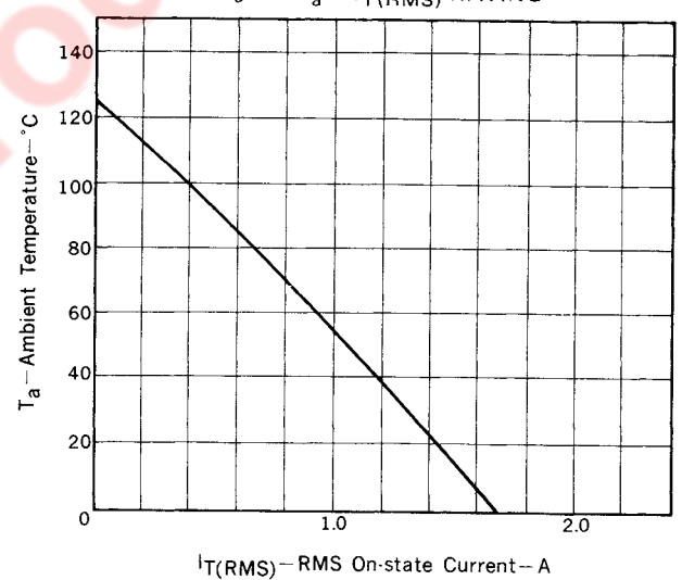
Fig. 12 T_a - I_T(\text{RMS}) RATING
