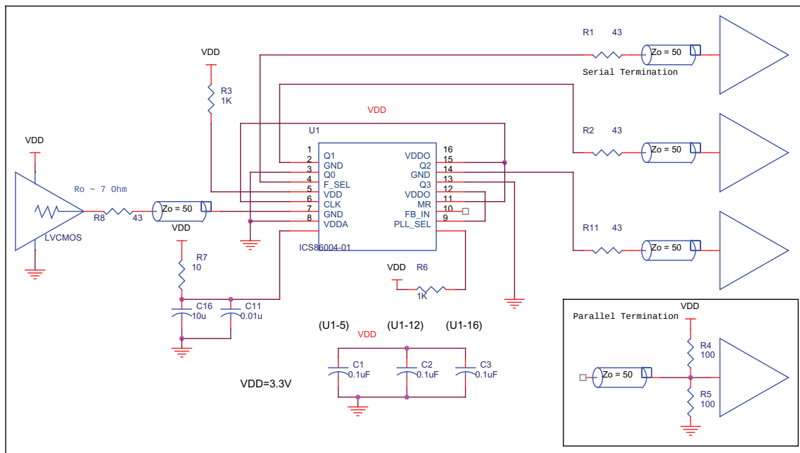
FIGURE 2. 86004-01 SCHEMATIC EXAMPLE
