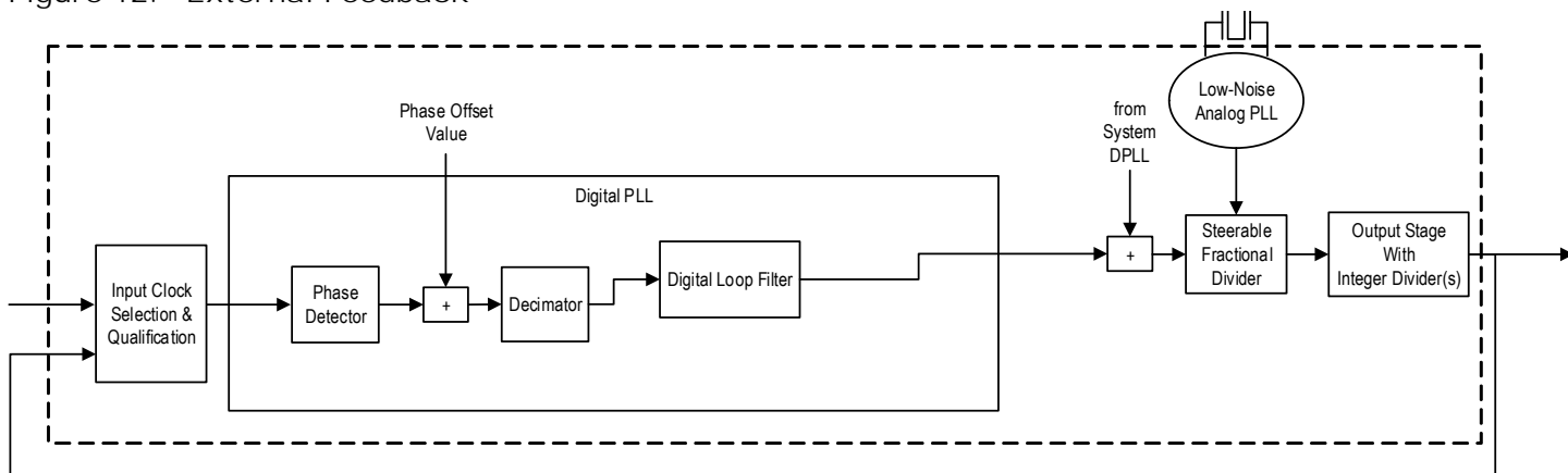
Figure 12. External Feedback
