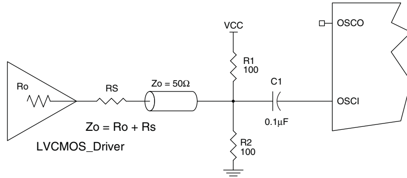
Figure 36. LVCMOS Driver to XTAL Input Interface
