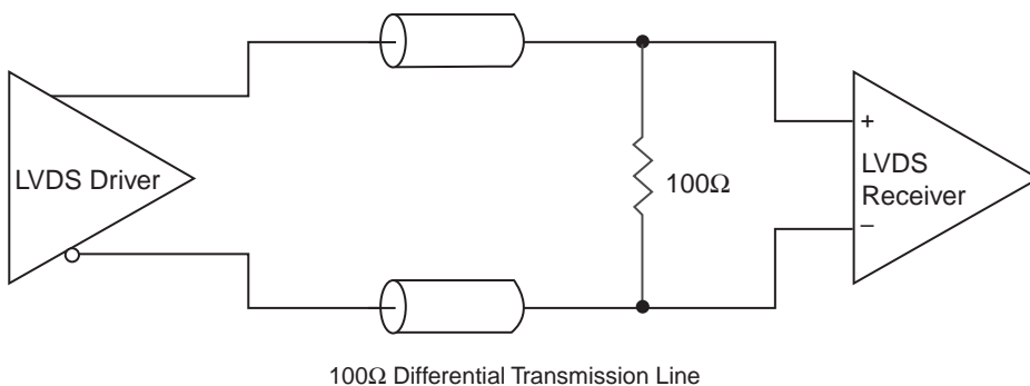
Figure 38. Standard LVDS Termination
