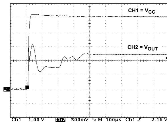
FIGURE 8. POWER-ON
