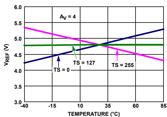
FIGURE 2. V_{OUT} vs TEMPERATURE ( A_V = 4 )
