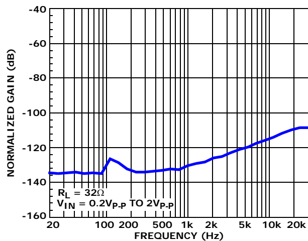
FIGURE 13. OFF-ISOLATION
