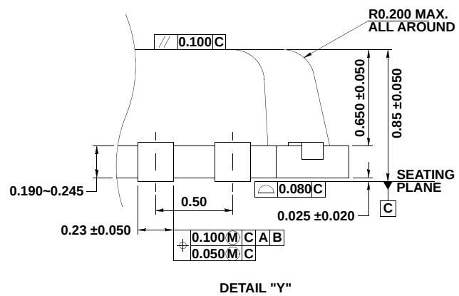
DETAIL "Y"
