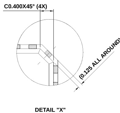
DETAIL "X"
