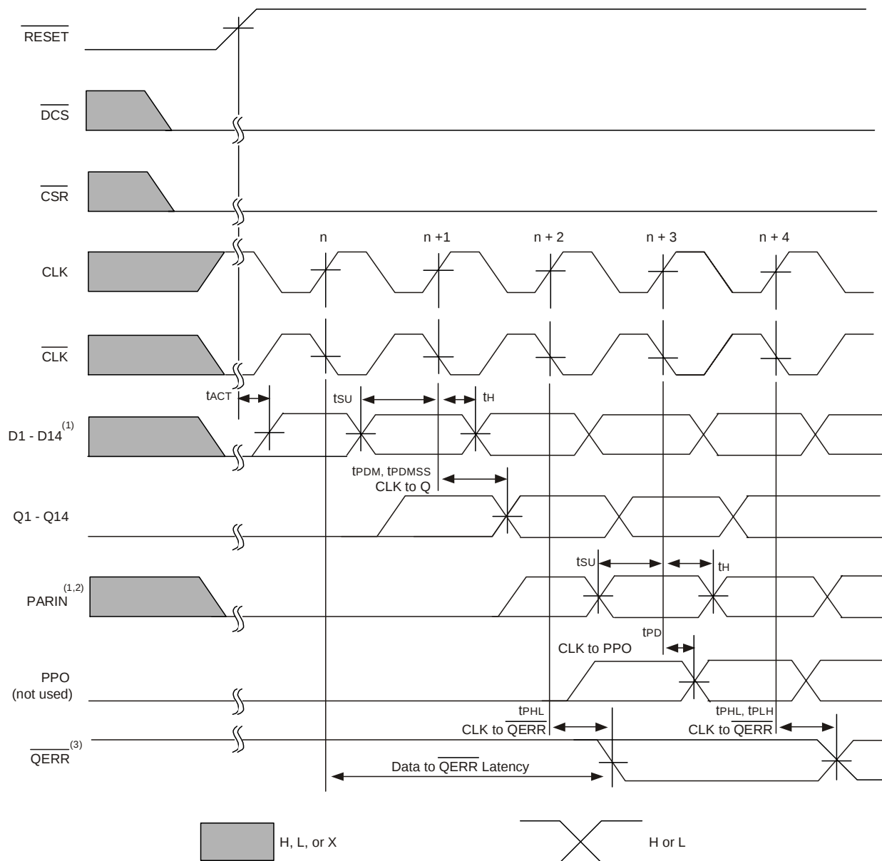
Timing Diagram for the Second SSTUAF32866B (1:2 Register-B Configuration) Device Used in a Pair; \text{C0} = 1 , \text{C1} = 1 , \overline{\text{RESET}} Switches from L to H
