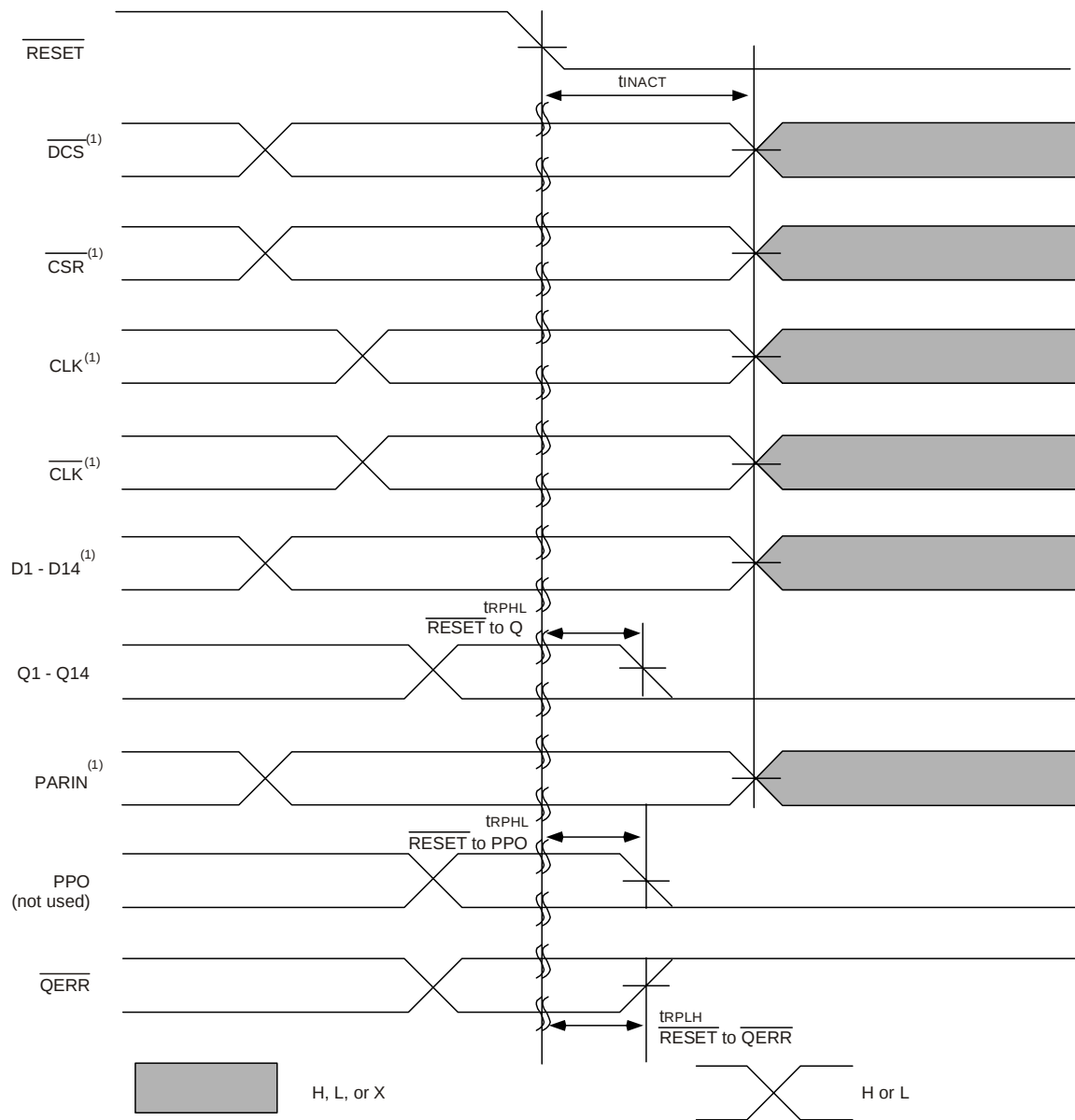
Timing Diagram for the First SSTUAF32866B (1:2 Register-A Configuration) Device Used in a Pair; C0 = 1, C1 = 1; RESET Switches from H to L
