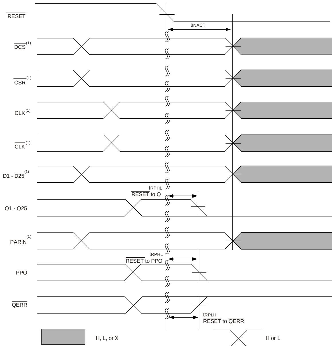
Timing Diagram for SSTUAF32866B Used as a Single Device; C0 = 0, C1 = 0, RESET Switches from H to L
