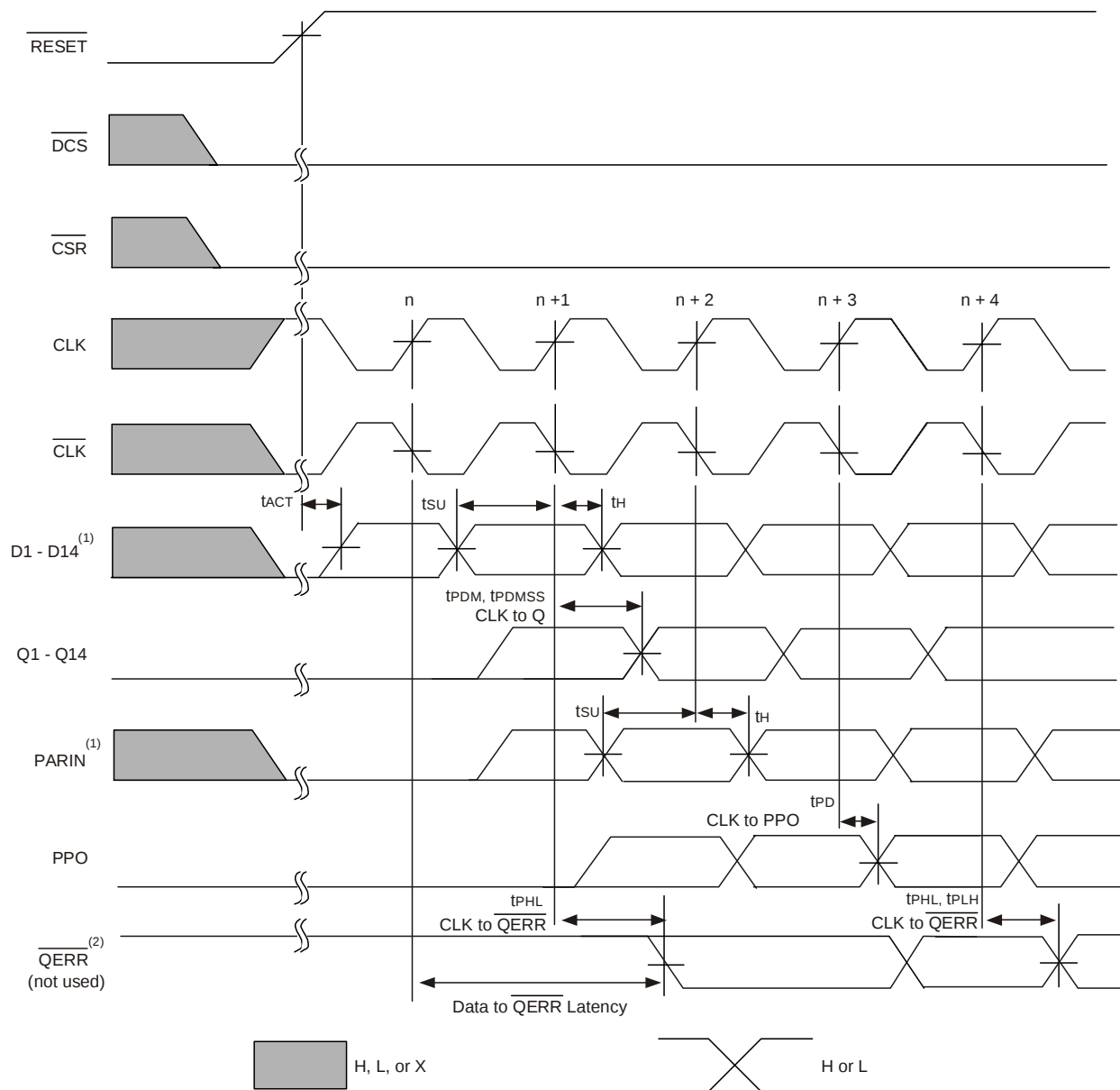
Timing Diagram for the First SSTUAF32866B (1:2 Register-A Configuration) Device Used in a Pair; C0 = 0, C1 = 1, \overline{RESET} Switches from L to H
