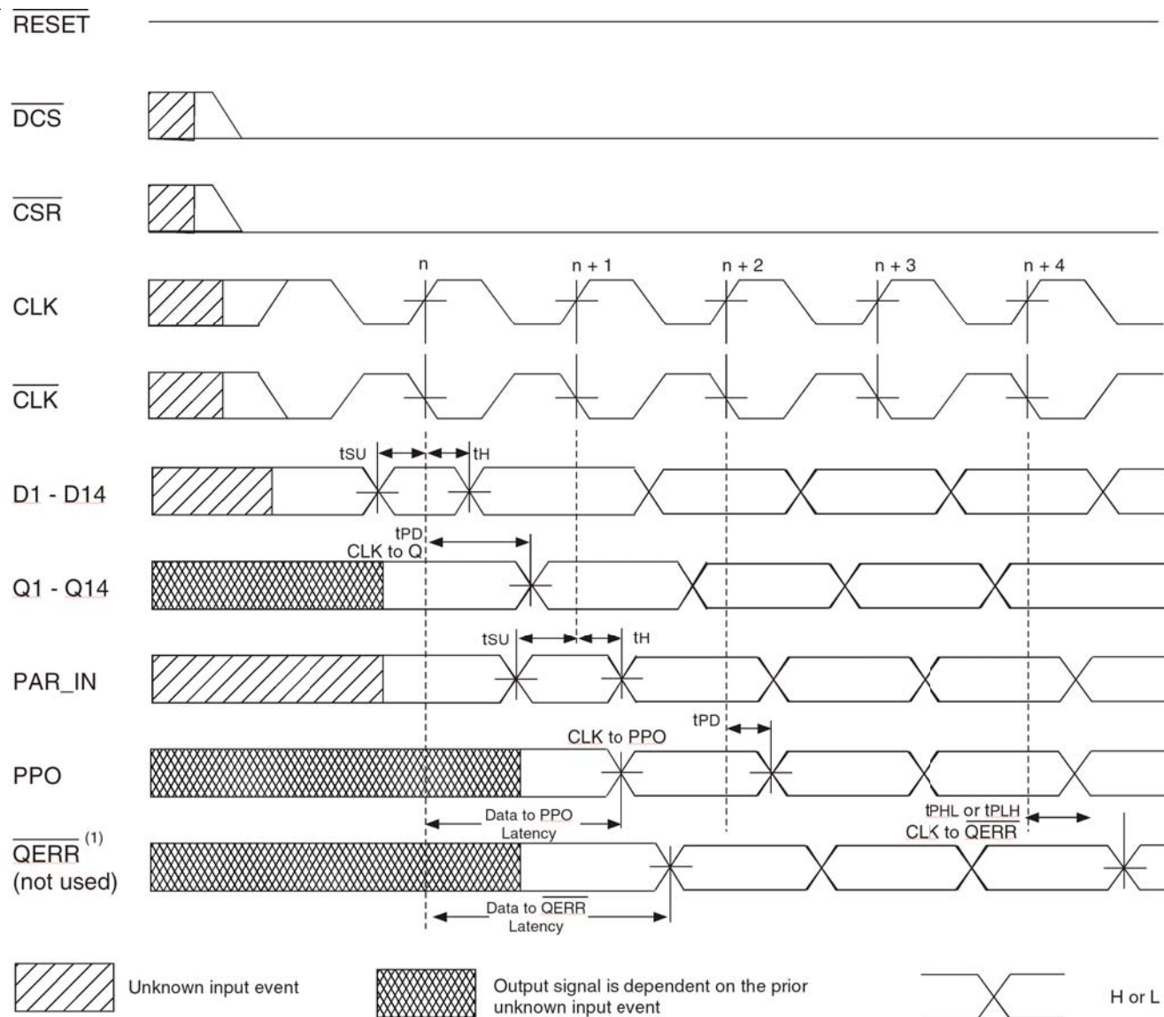
Figure 16 Timing diagram for the second SSTU32866 (1:2 register-B configuration) device used in pair: \text{C0} = 1 , \text{C1}=1 ; \overline{\text{RESET}} being held HIGH
