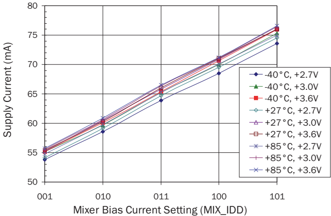
Operating Current, One Mixer Enabled versus Temperature and Supply Voltage
