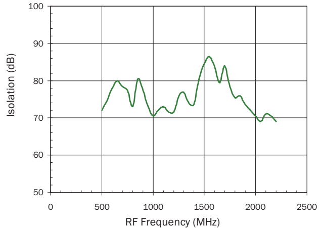
Full Duplex Mode Typical Isolation Between Mixers
