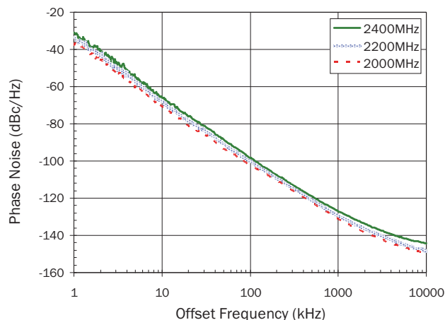
VC02 Open Loop Phase Noise
