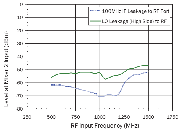
Full Duplex Mode Typical Isolation Between Mixers
