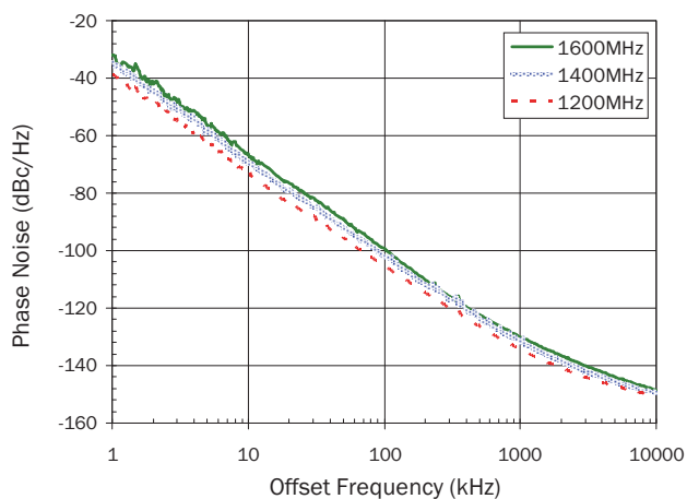
VC03 Open Loop Phase Noise
