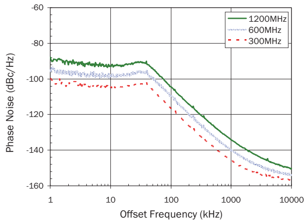
VC03 With Passive Loop Filter
