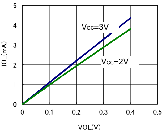
V_{OL} vs. I_{OL} ( \overline{INTR} pin) (Except R2262Txx) ( T_a=25^{\circ}\text{C} )
