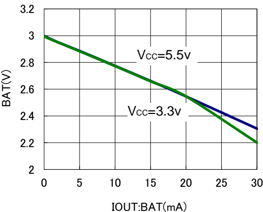
BAT vs. Output load Current ( I_{OUT:BAT} ) ( T_a=25^{\circ}\text{C} )
