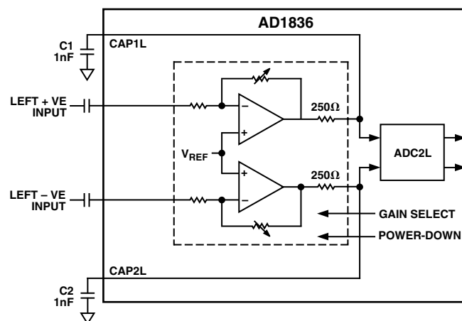
Figure 13. Differential Mode
