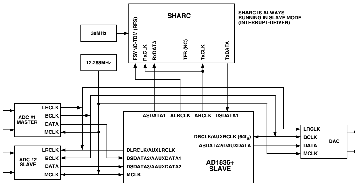
Figure 10. AUX-Mode Connection to SHARC (Slave Mode)
