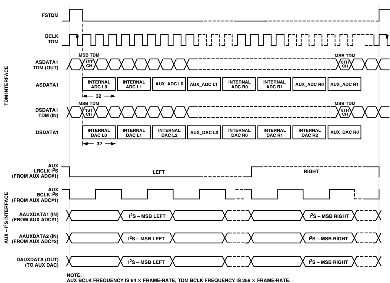
Figure 8. AUX-Mode Timing
