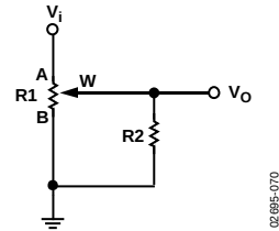
Figure 70. Resistor Scaling with Log Adjustment Characteristics
