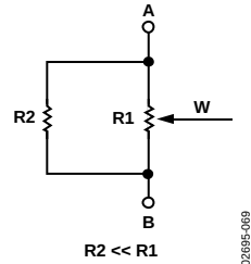
Figure 69. Lowering the Nominal Resistance
