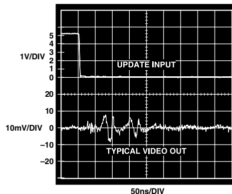
TPC 10. Switching Transient (Glitch)
