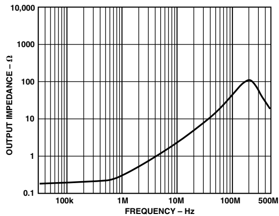
TPC 12. Output Impedance, Enabled
