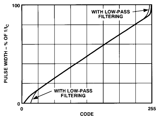
Figure 5. Transfer Function
