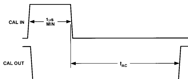
Figure 3. AutoCAL Timing
