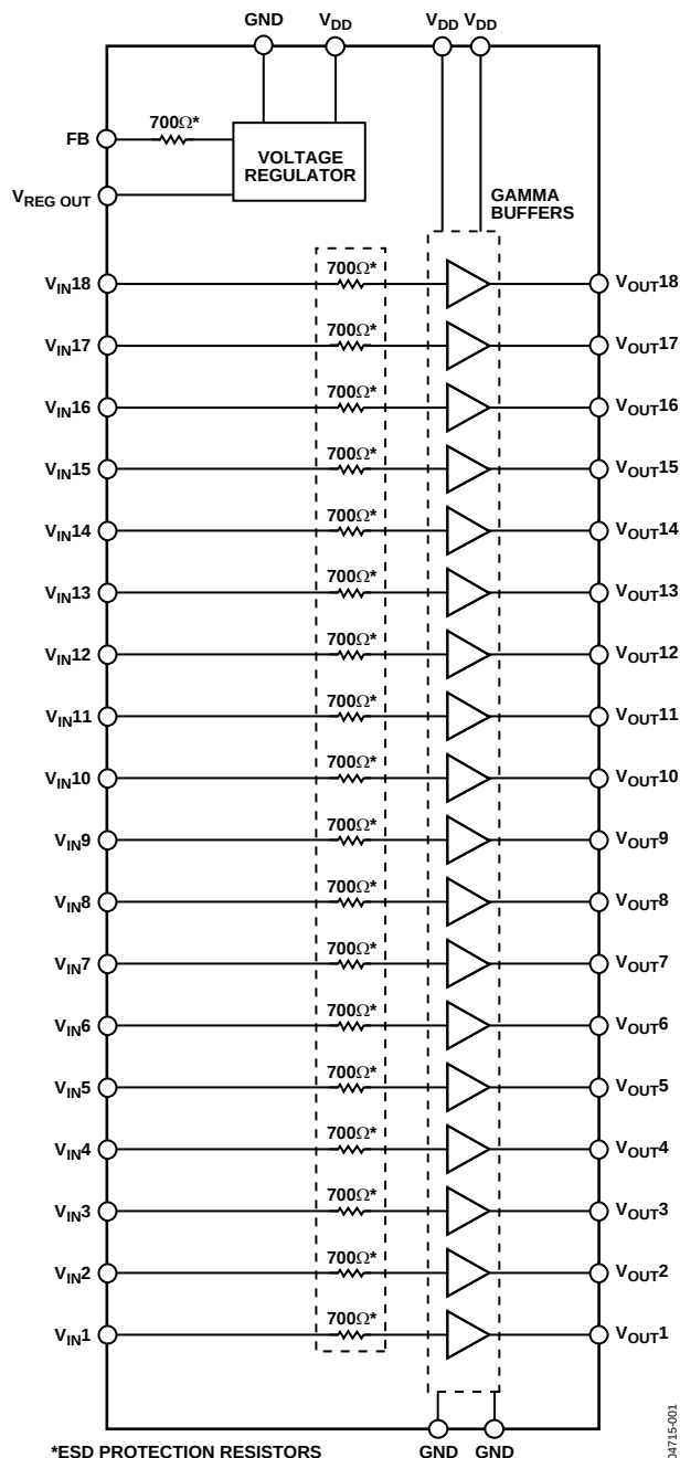
Figure 1. 48-Lead LQFP
