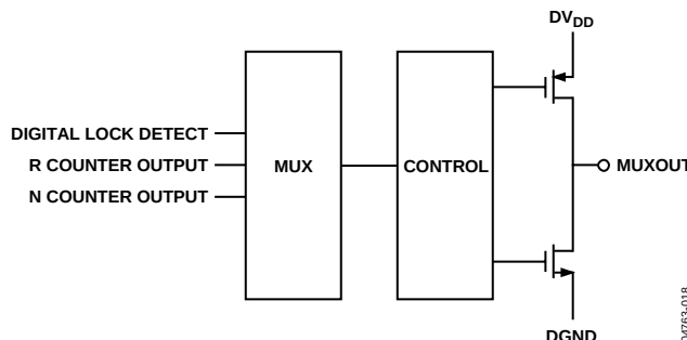
Figure 18. MUXOUT Circuit
