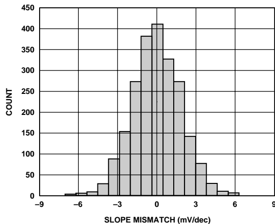
Figure 30. Distribution of Channel-to-Channel Slope Mismatch ( V_{Y1} - V_{Y2} )
