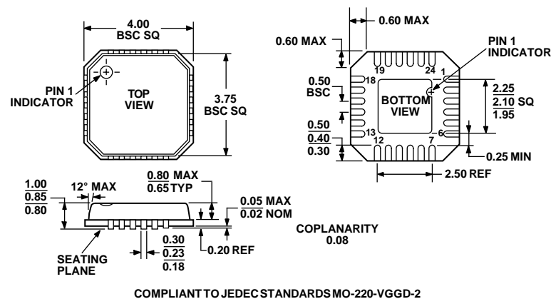
Figure 43. 24-Lead Lead Frame Chip Scale Package [LFCSP] (CP-24) Dimensions shown in millimeters
