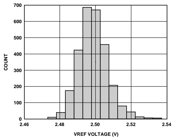
Figure 29. Distribution of V_{REF} ( R_L = 100\text{ k}\Omega )
