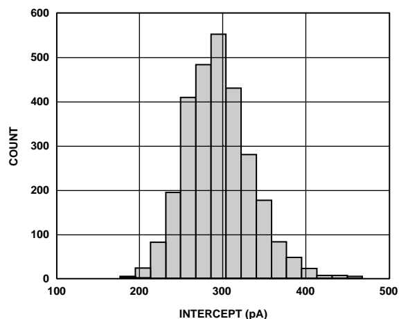
Figure 28. Distribution of Logarithmic Intercept
