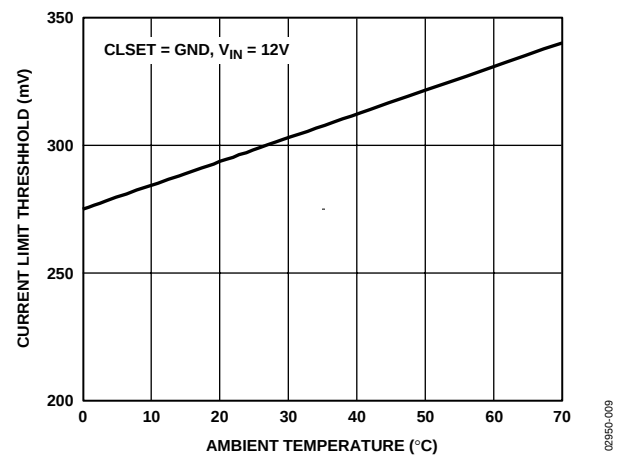
Figure 9. Current Limit Threshold vs. Temperature
