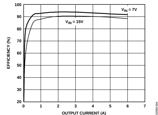
Figure 4. Efficiency vs. 5 V Output Current
