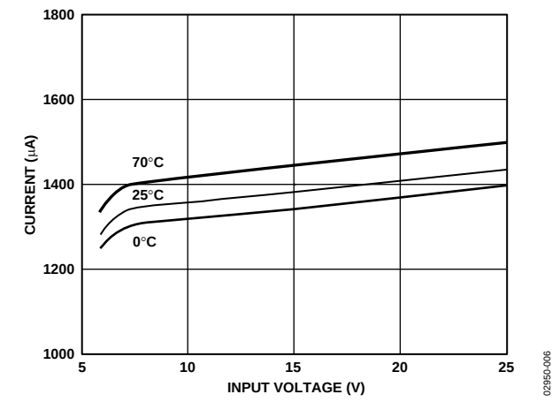
Figure 6. Input Standby Current vs. Input Voltage
