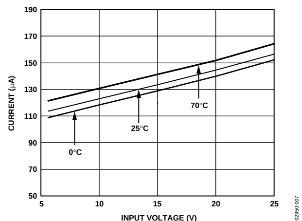
Figure 7. Input Shutdown Current vs. Input Voltage
