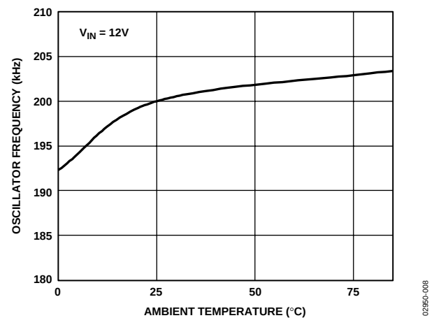
Figure 8. Oscillator Frequency vs. Temperature
