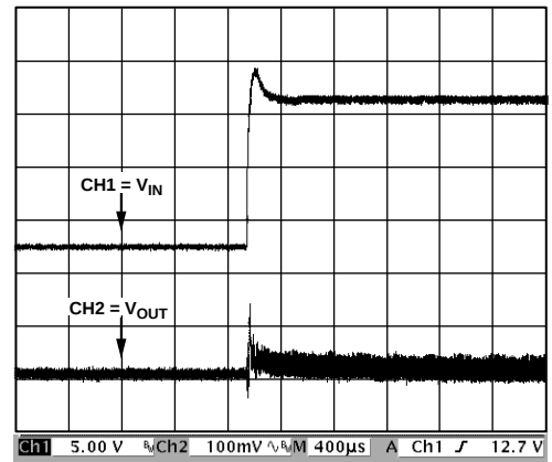
Figure 14. V_{IN} = 7.5 \text{ V} to 22 \text{ V} Transient, 5 \text{ V} Output, CH1—Input Voltage, CH2—Output Voltage
