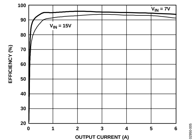
Figure 5. Efficiency vs. 3.3 V Output Current
