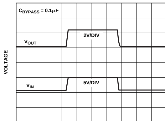
TPC 33. ADR391 Turn-On/Turn-Off Response at 5 V
