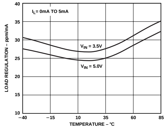
TPC 10. ADR391 Load Regulation vs. Temperature
