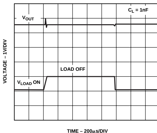
TPC 29. ADR391 Load Transient Response
