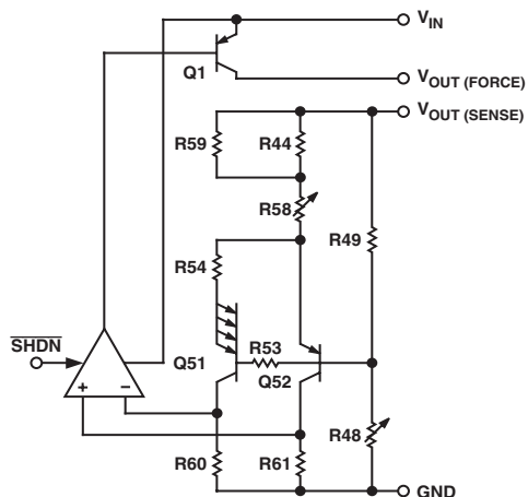
Figure 2. Simplified Schematic
