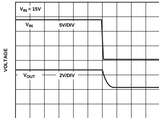
TPC 32. ADR391 Turn-Off Response at 15 V
