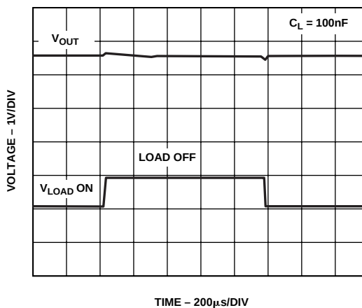
TPC 30. ADR391 Load Transient Response
