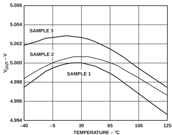
TPC 4. ADR395 Output Voltage vs. Temperature
