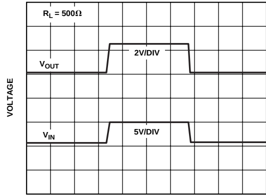
TPC 34. ADR391 Turn-On/Turn-Off Response at 5 V
