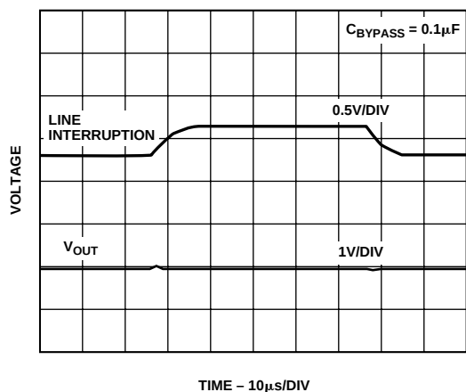
TPC 27. ADR391 Line Transient Response
