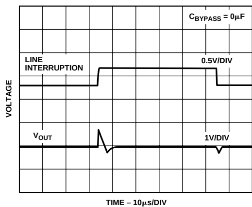
TPC 26. ADR391 Line Transient Response
