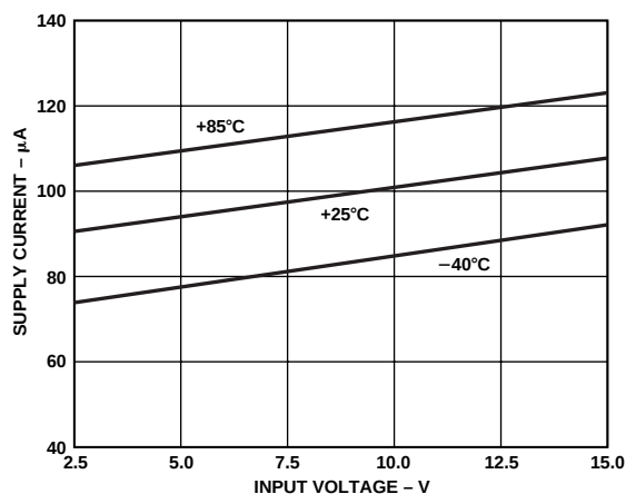
TPC 5. ADR390 Supply Current vs. Input Voltage
