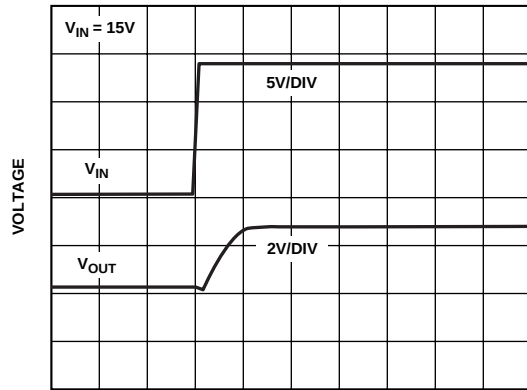
TPC 31. ADR391 Turn-On Response Time at 15 V
