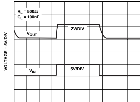
TPC 35. ADR391 Turn-On/Turn-Off Response at 5 V
