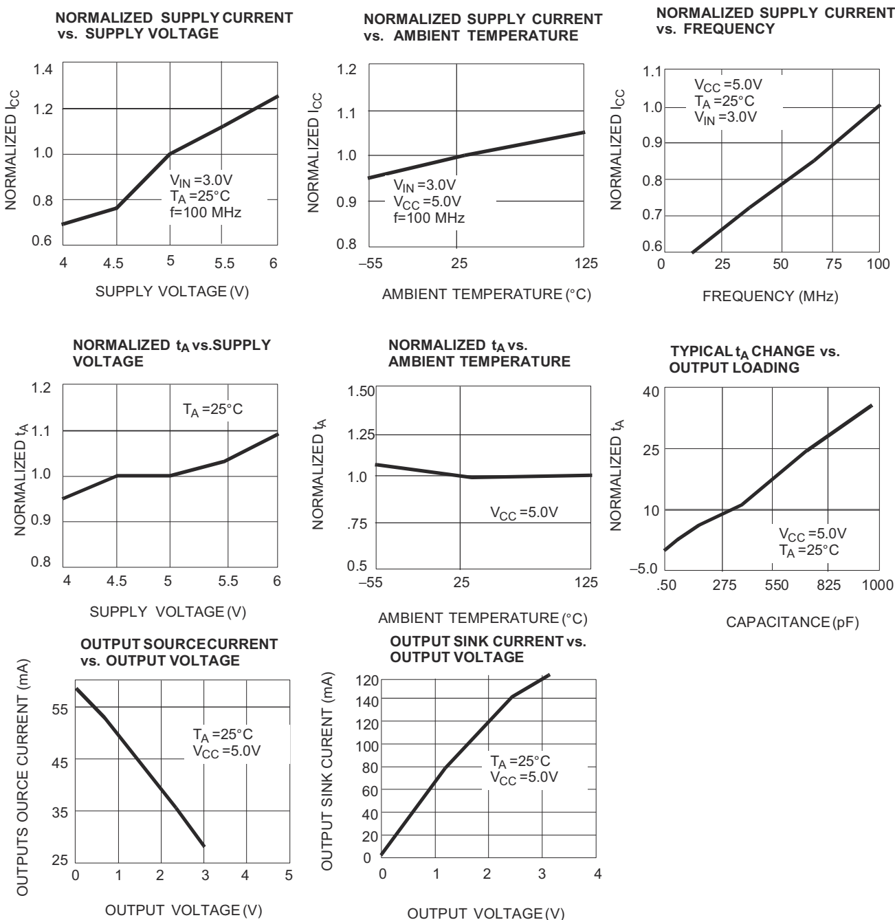
Figure 23. Typical AC and DC Characteristics
