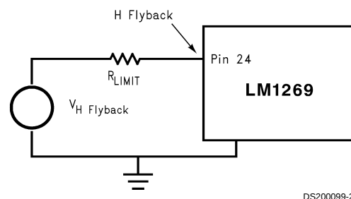
FIGURE 5. H Flyback Input Pulse
