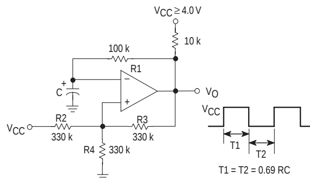
Figure 8. Squarewave Oscillator
