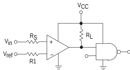
Figure 7. Driving Logic
