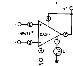
Fig. 17 - Comparator and solenoid driver.
