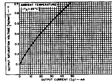
Fig. 13 - Output saturation voltage vs. output current.
