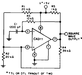
Fig. 26 - 100-kHz free-running multivibrator.
