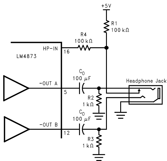
FIGURE 3. Headphone Circuit
