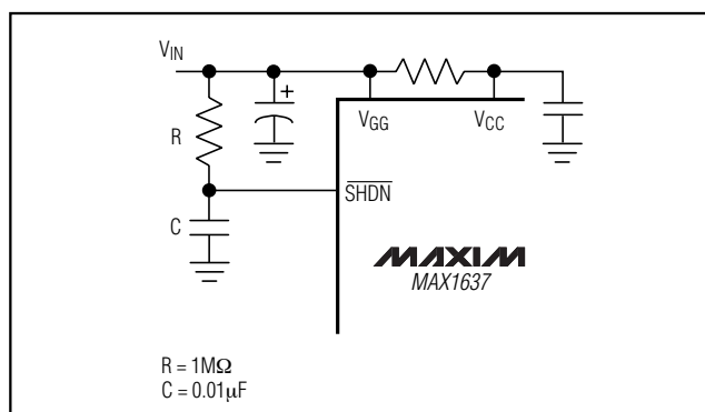
Figure 5. Power-On Reset RC Network for Automatic Start-Up
