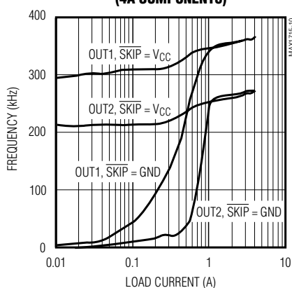
FREQUENCY vs. LOAD CURRENT (4A COMPONENTS)
