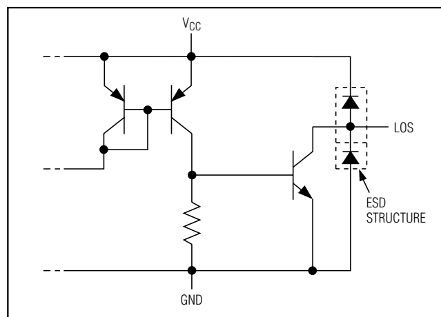
Figure 6. MAX3748A/MAX3748B LOS Output Circuit
