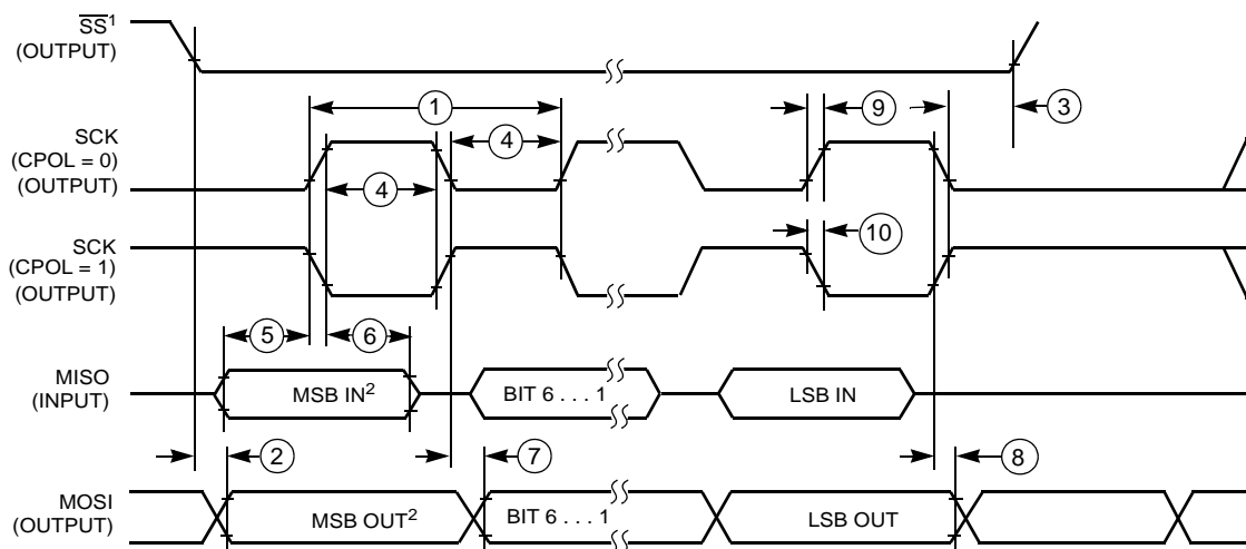
Figure 33. SPI Master Timing (CPHA = 0)
