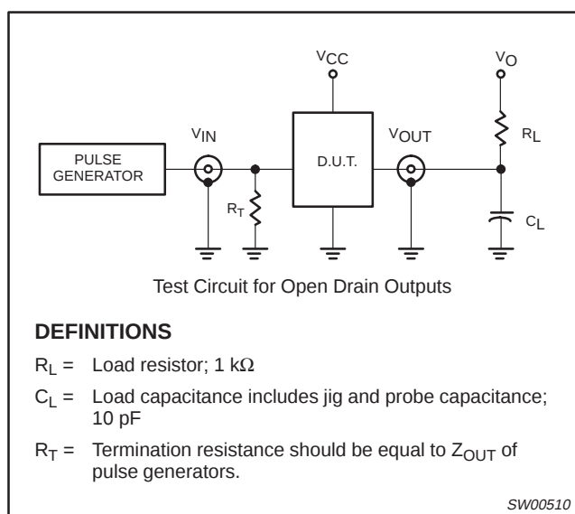
Figure 14. Test circuit
