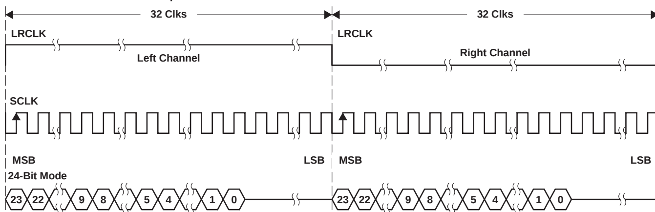
Figure 2-5. Left-Justified 64-Fs Format
