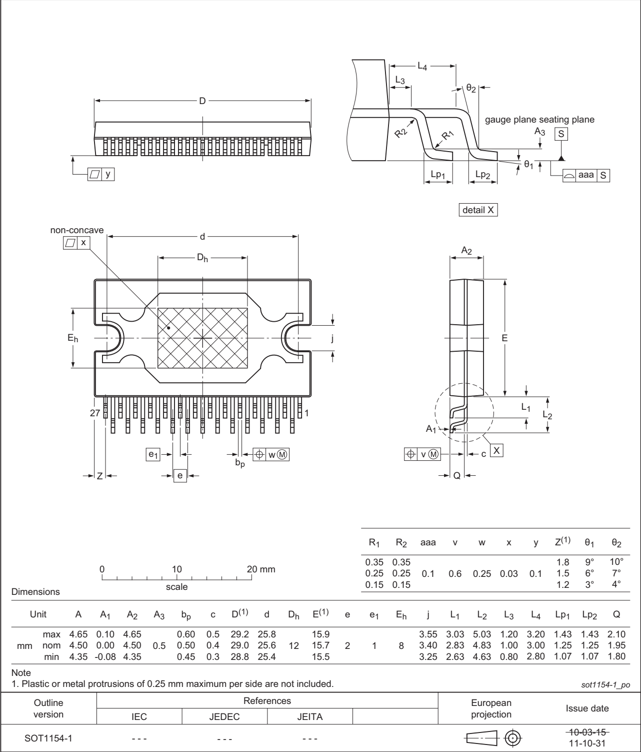
Fig 45. Package outline SOT1154-1 (DBSMS27P)
