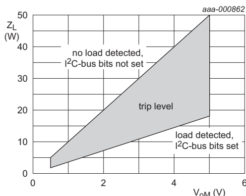
Fig 20. AC-load impedance as a function of peak output voltage (low current AC-load detection)
