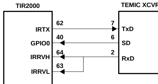
Figure 6–3. Temic Transceivers
