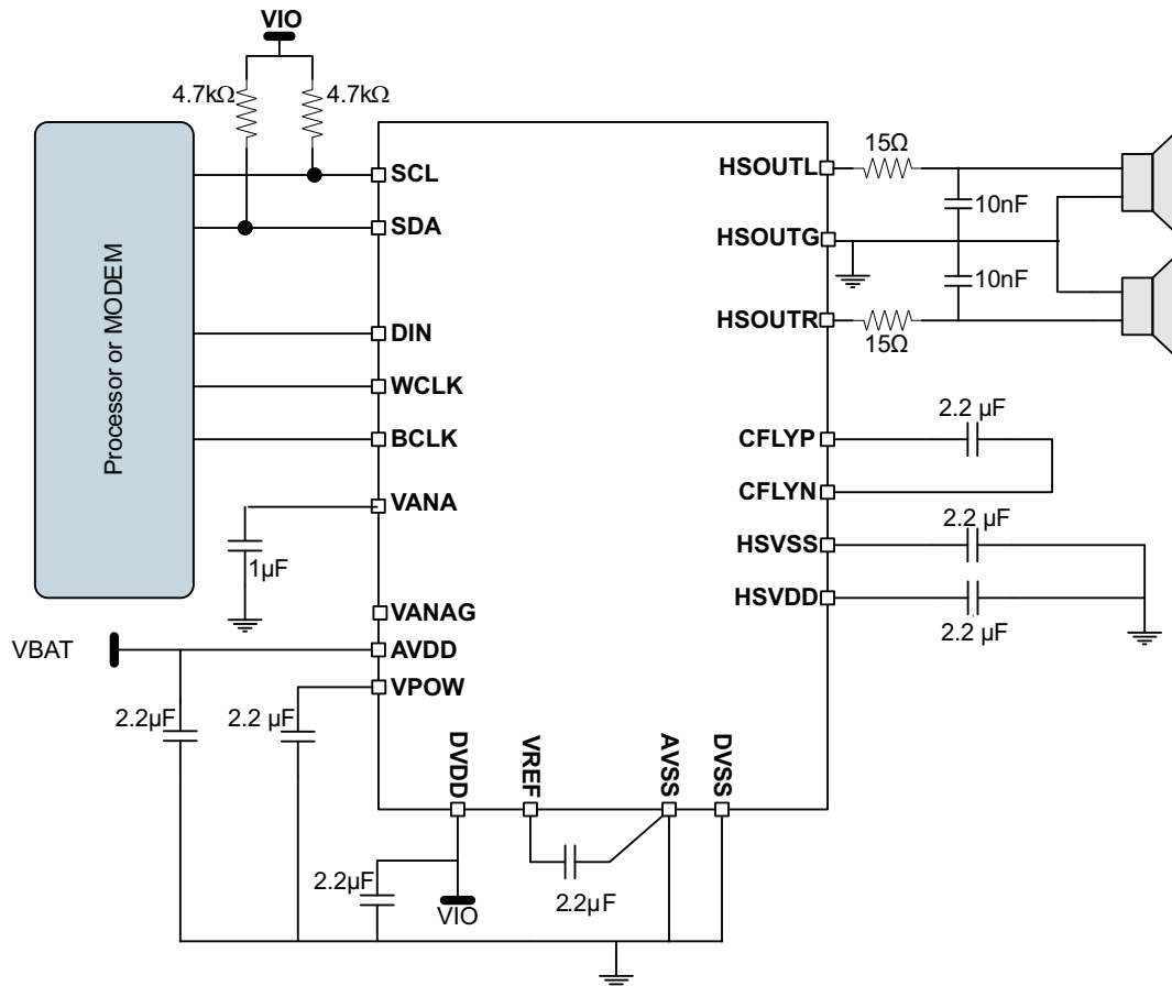
Figure 13. Typical Circuit
