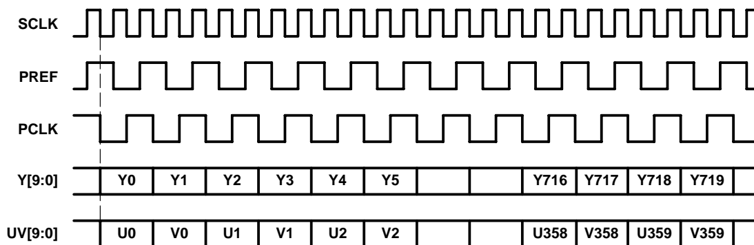
Figure 2–23. 20-Bit 4:2:2 Output Format
