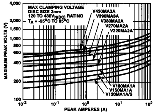
FIGURE 4. CLAMPING VOLTAGE FOR V120MA1A/S - V430MA3A
