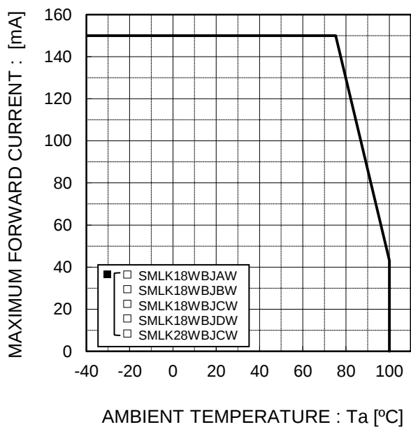
Fig.4 Derating
